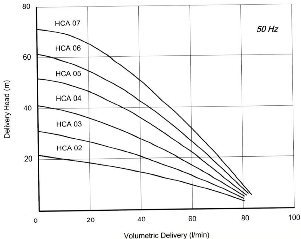
Performance Curve
