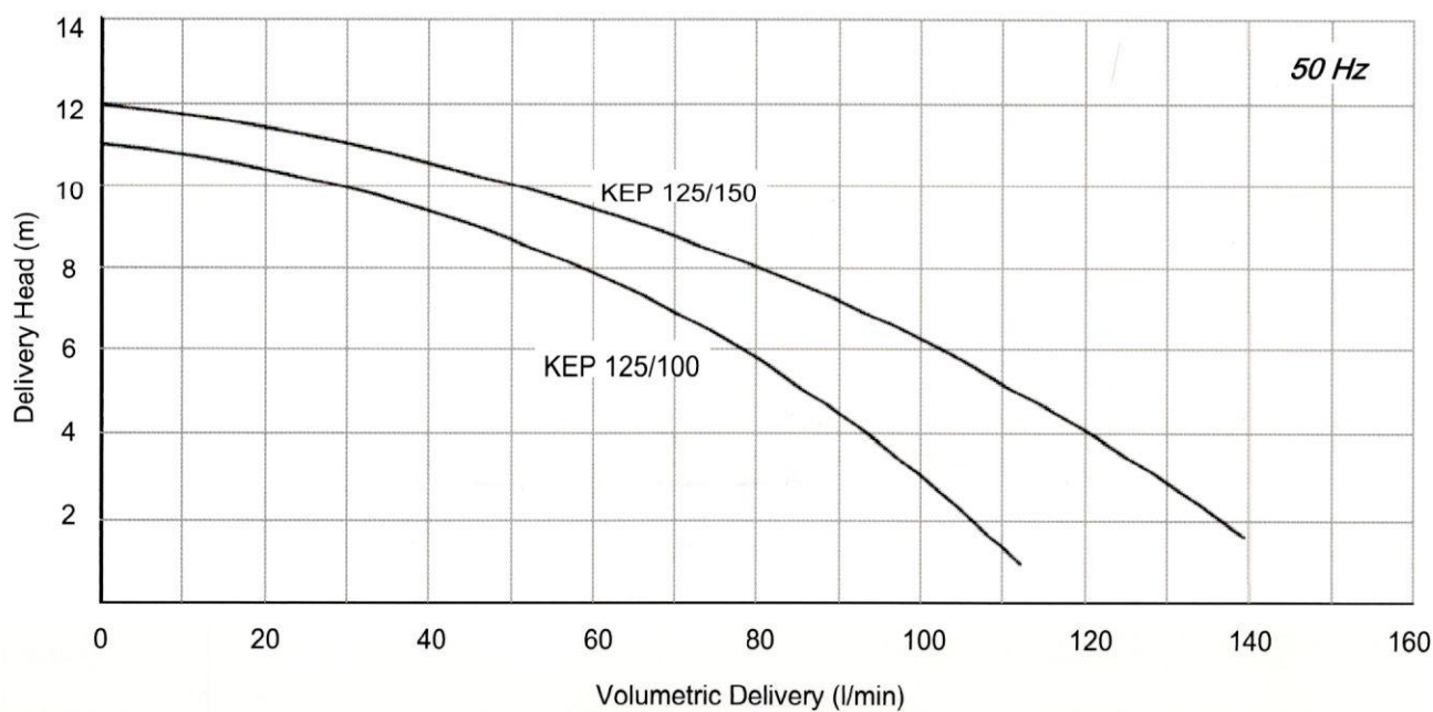
Performance Curve
